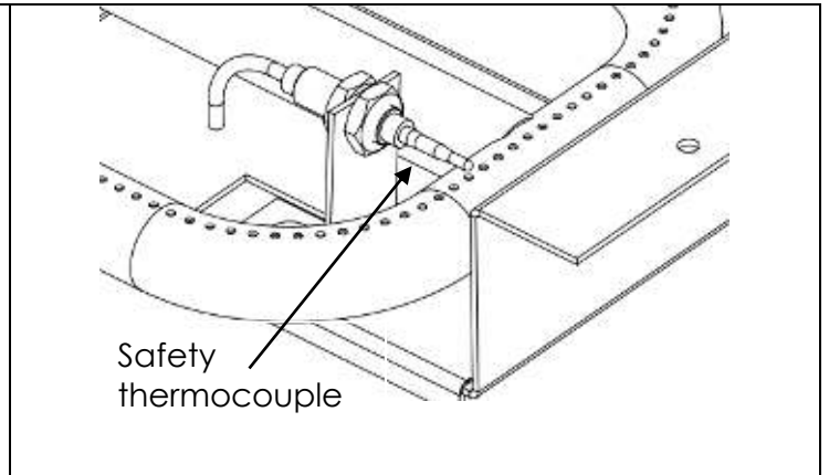
FIGURE 5 – THERMOCOUPLE SAFETY
