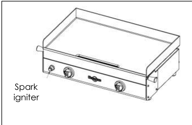
FIGURE 4 – PIEZO ELECTRIC
